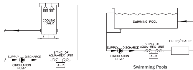
Re-Circulating Systems
